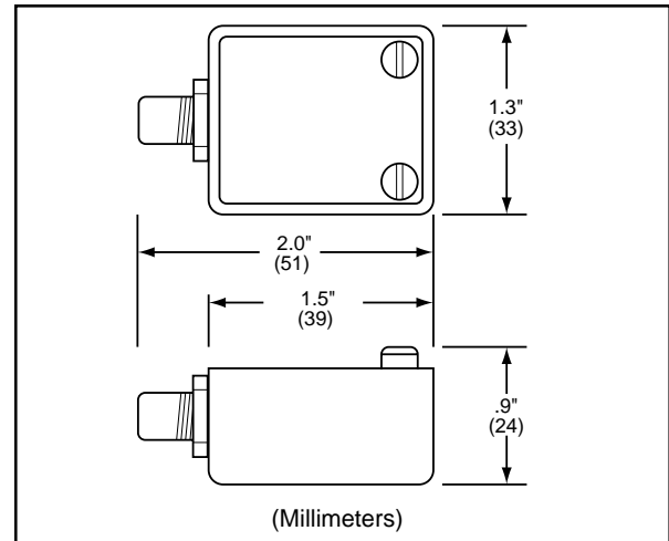
AS1000 Drawing
